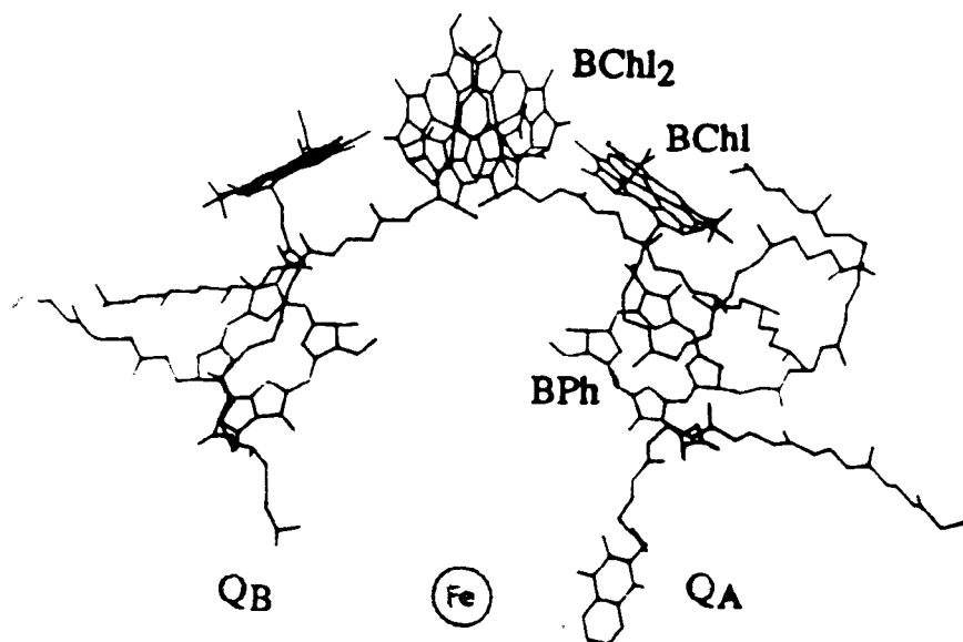
Figure II. Redox-active species involved in the initial charge separation for a photosynthetic bacterium (cf Deisenhofer et al, ref. 3, and Yeates et al, ref. 3), with labels added, to conform to the present text; they include a missing Q_b .
