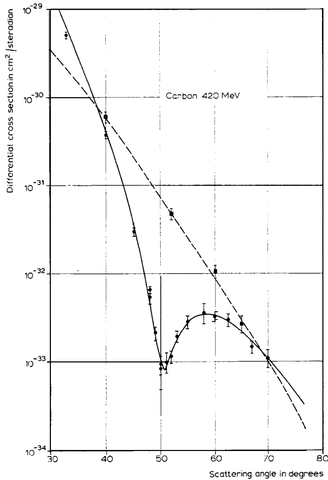
Fig. 5. This figure shows the elastic and inelastic curves corresponding to the scattering of 420-MeV electrons by ^{12}\text{C} . The solid circles, representing experimental points, show the elastic-scattering behavior while the solid squares show the inelastic-scattering curve for the 4.43-MeV level in carbon. The solid line through the elastic data shows the type of fit that can be calculated by phase-shift theory for the model of carbon shown in Fig. 8.
