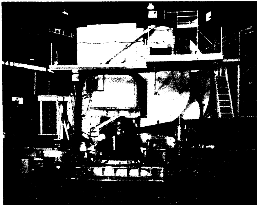
Fig. 3. A recent photograph of the double-spectrometer system is shown in this figure. The shield of the smaller spectrometer can be removed easily with the aid of an auxiliary stand, not shown in the photograph. The long tube in the foreground is the vacuum pipe leading to the Faraday cup, which is not visible in the photograph.
