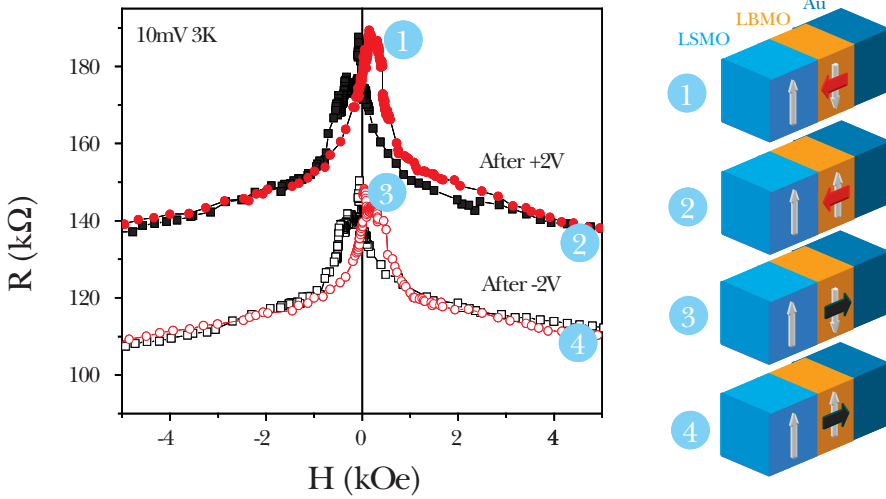
Figure 9. Four state resistance of a tunnel junction composed of a biferric tunnel barrier ( \text{La}_{0.1}\text{Bi}_{0.9}\text{MnO}_3 ) between a ferromagnetic electrode of \text{La}_{2/3}\text{Sr}_{1/3}\text{MnO}_3 and a nonmagnetic electrode of gold. The states 1-4 correspond to the magnetic (white arrows) and electric (black arrows) polarizations represented on the right of the figure. From Gajek et al. 44 .
