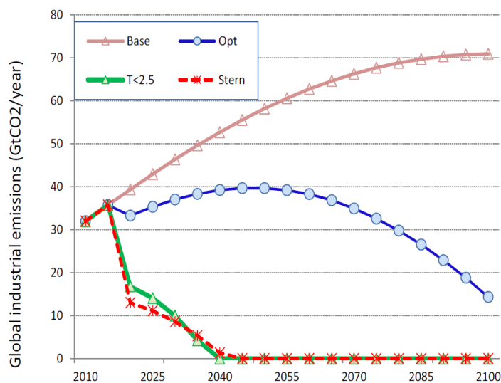
Figure 3: Emissions of CO 2 in four scenarios. Predictions from DICE-2016R2.
